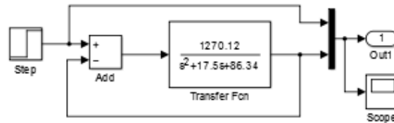
Fig.3 The Simulation Model Diagram of System
