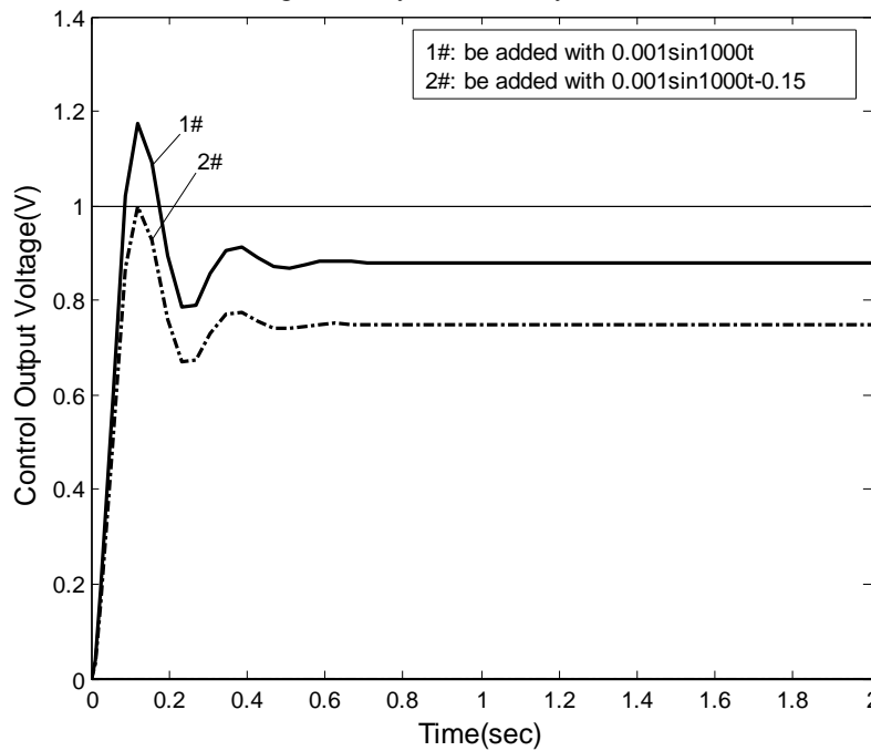
Fig.6 The Simulation Results of System with Cylinder Friction Force Compensation
