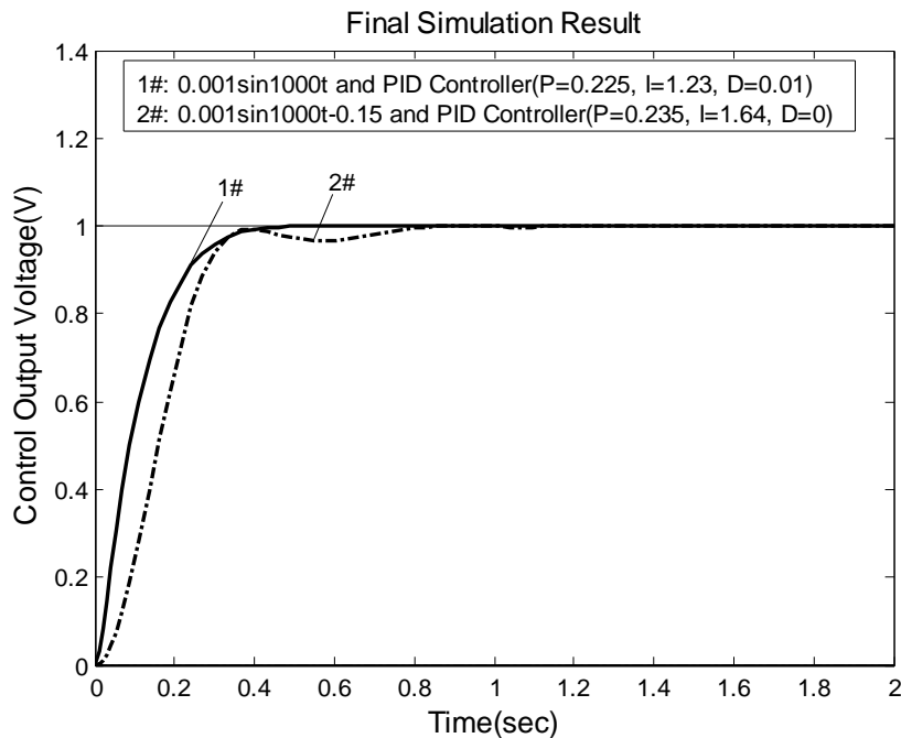
Fig.8 The Simulation Results of System by PID Control
