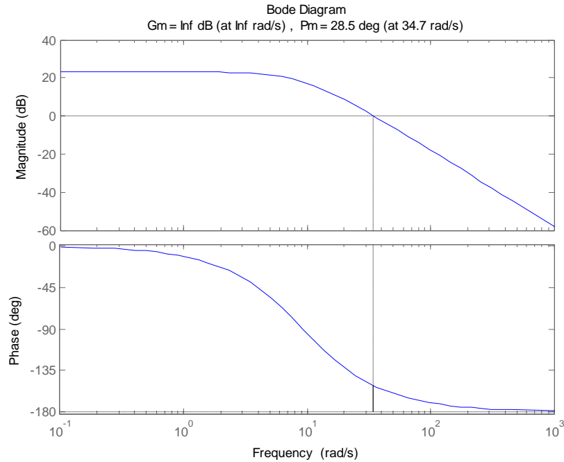
Fig.5 Bode Diagram
